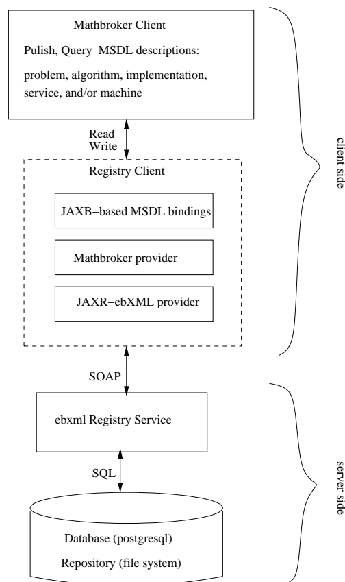
Figure 8: MathBroker Registry Architecture
